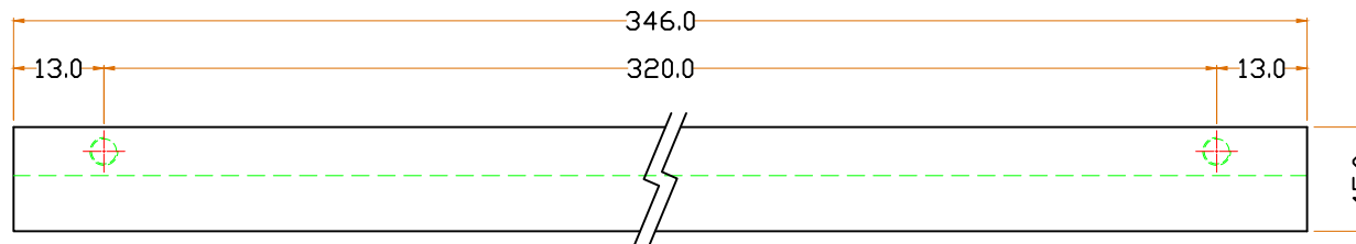
FRONT VIEW
