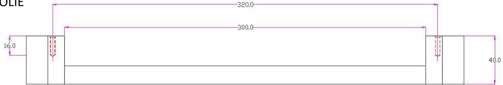
TOP VIEW
