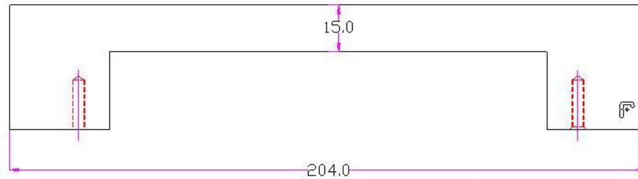
BOTTOM VIEW
