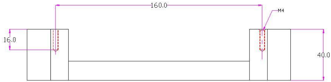
TOP VIEW
