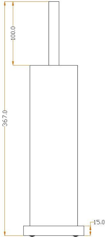
FRONT VIEW
